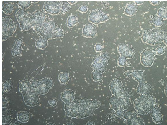
CiRA-j-1489-D: passage-3
