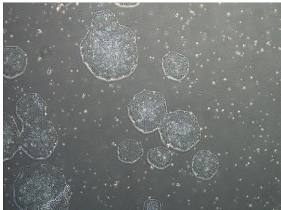
CiRA-j-1489-F: passage-3
