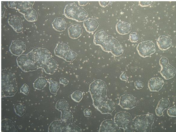
CiRA-j-1489-C: passage-3
