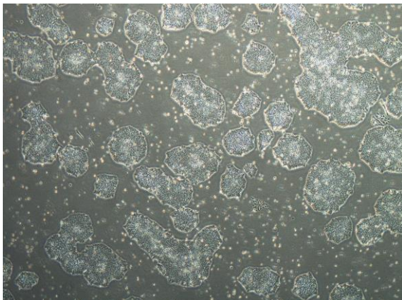
CiRA-j-1489-E: passage-3
